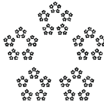
n = 5, r = 1/3
