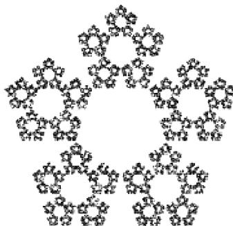
n = 5, r = 3/8
